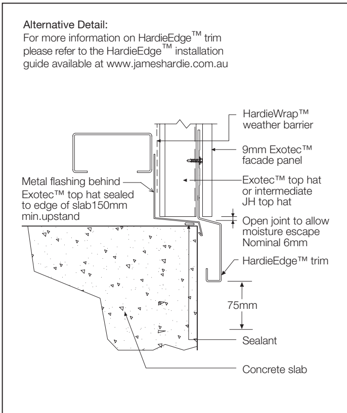
FIGURE 17B WALL BASE TYPICAL DETAIL 2 WITH HARDIEEDGE™ TRIM
