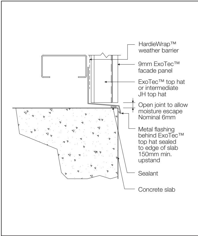
FIGURE 17A WALL BASE TYPICAL DETAIL 2
